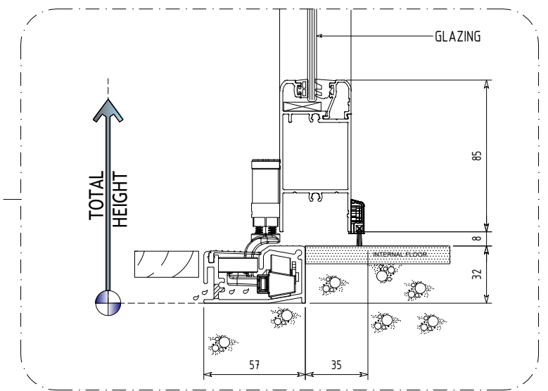
Recessed Channel Track OPTION
