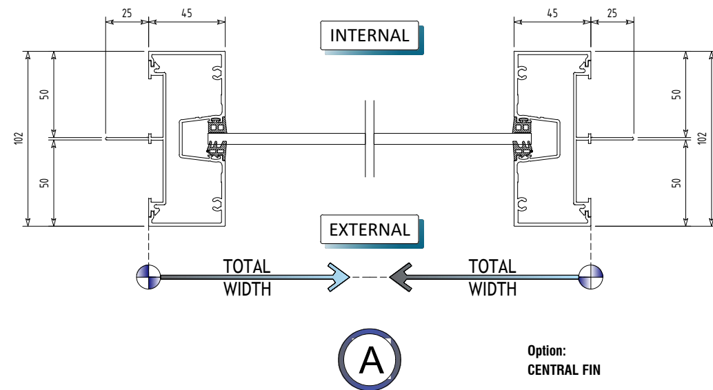
STANDARD DETAIL
