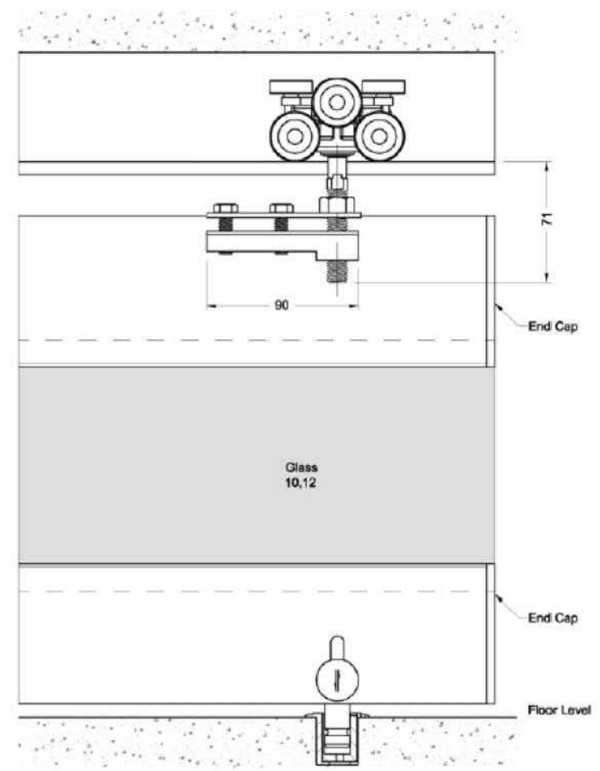
Sectional Elevation
